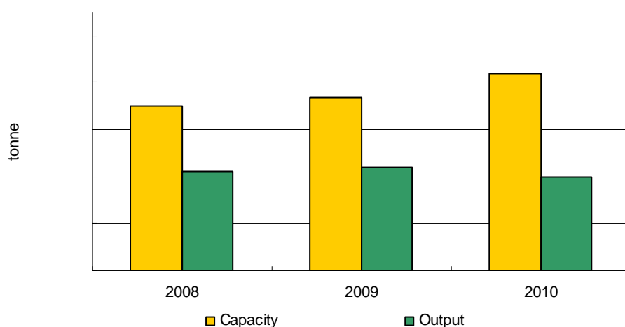
Figure 2.5.1-1 Capacity and output of mancozeb technical (Converted to 85% TC) in China, 2008-2010
