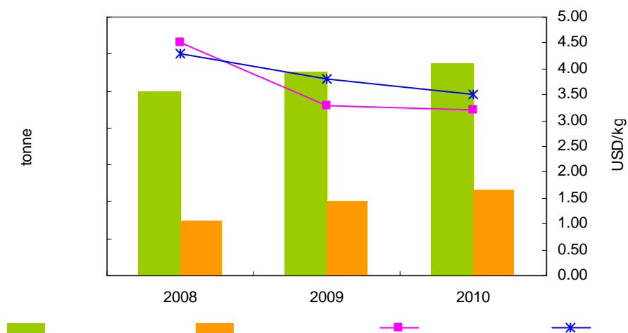
Figure 3.2-1 Export volume and price of mancozeb, 2008-2010
